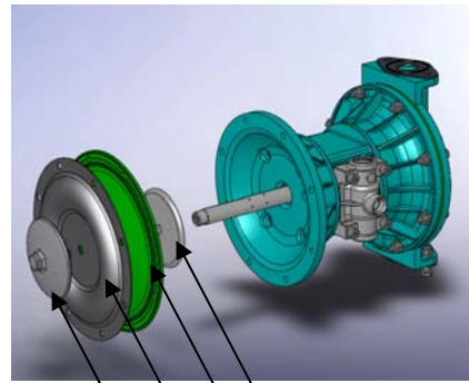
Front Plate Back Plate
