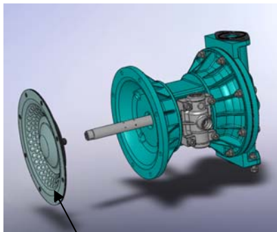
New One-Piece PTFE Extreme Diaphragm (No Additional Parts)
